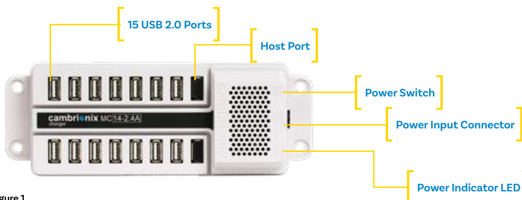
Figure 1 MultiCharger connections
